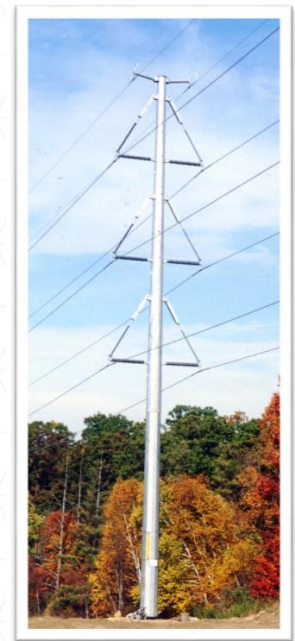
The new 120 kV monopoles will be similar to the one shown here.
